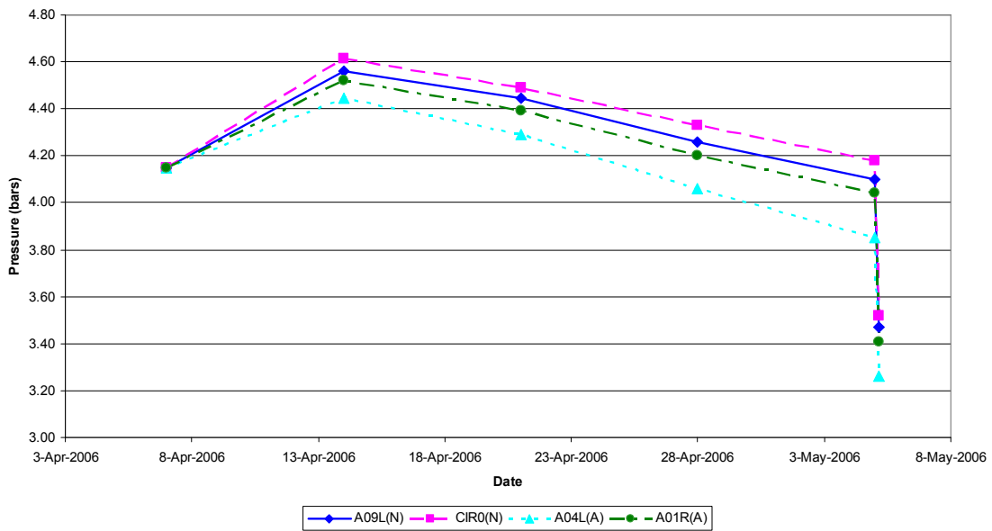
Figure 14: Measured inflation pressure change with time in Sleak test for T125/70D15 MINI SPARE 95M
